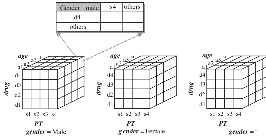
Figure 3 An example a 4-D contingency cube, C[Age, Gender, Drug, PT] .
